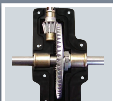
Fully Enclosed Metal Gears with Zerk Fittings
